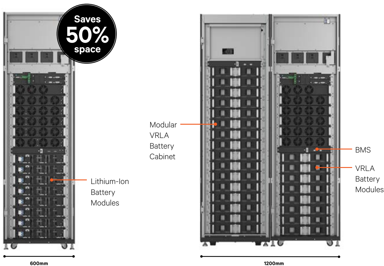
Vertiv™ Liebert® APM2 10-120kW with modular internal Lithium-Ion batteries
