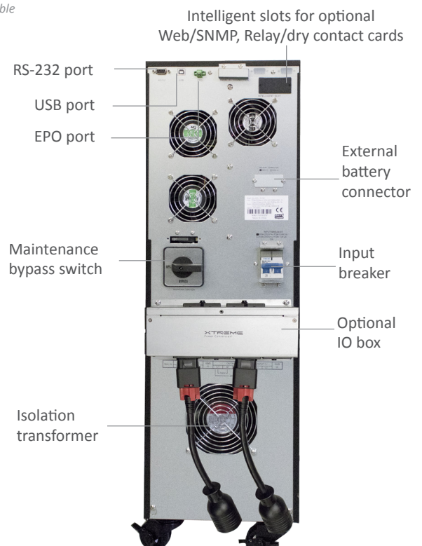
TX91 rear view
