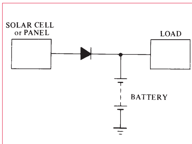
Figure 10. Block Diagram of a Solar System
