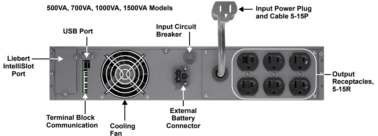
Figure 3 Liebert® GXT3™ 120V rack/tower models—rear panel components
