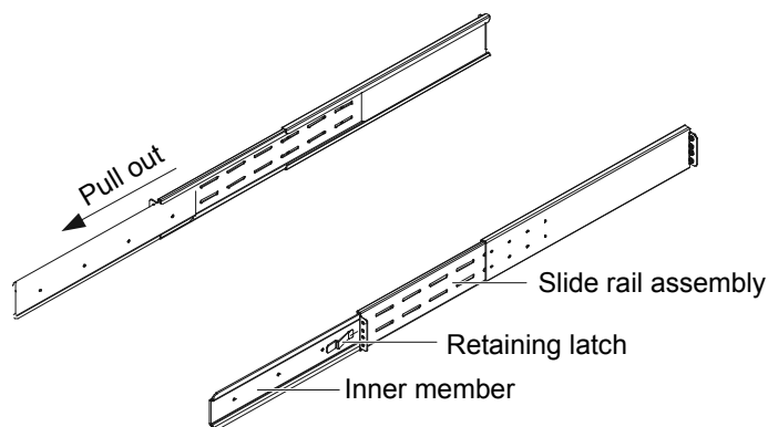
Figure 11 Pulling inner member from each slide rail assembly
