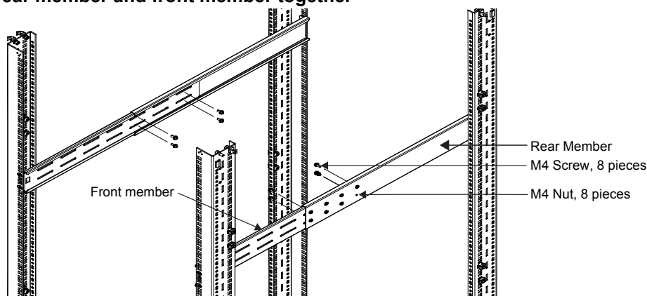
Figure 14 Fastening rear member and front member together
