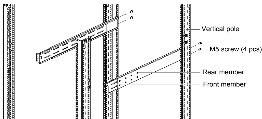
Figure 12 Installing rear member of each slide rail assembly
