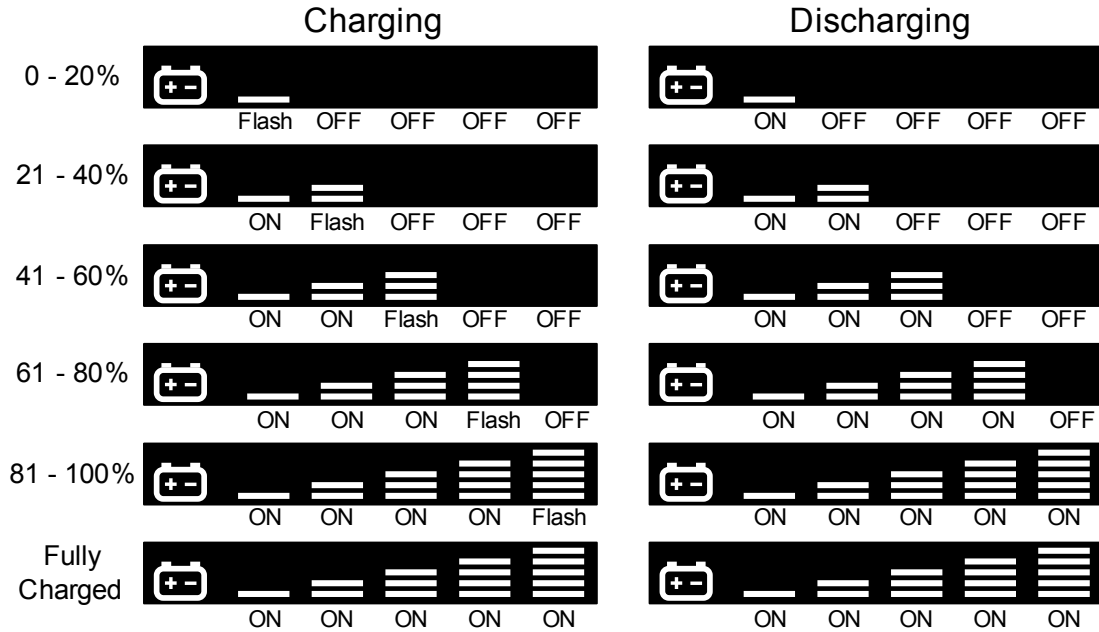
Figure 19 Battery level indicators
