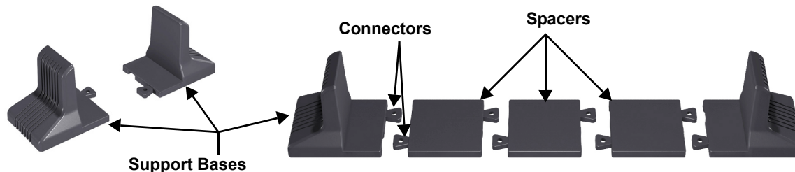
Figure 7 Support bases
