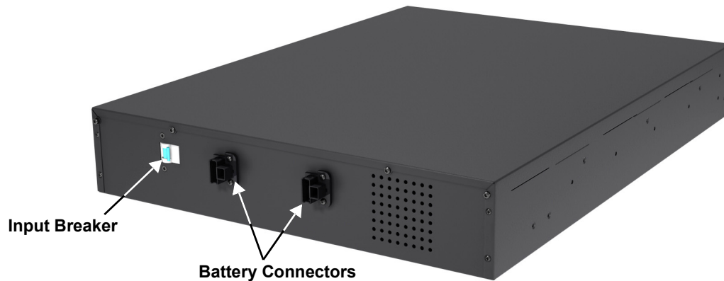
Figure 26 Battery cabinet
