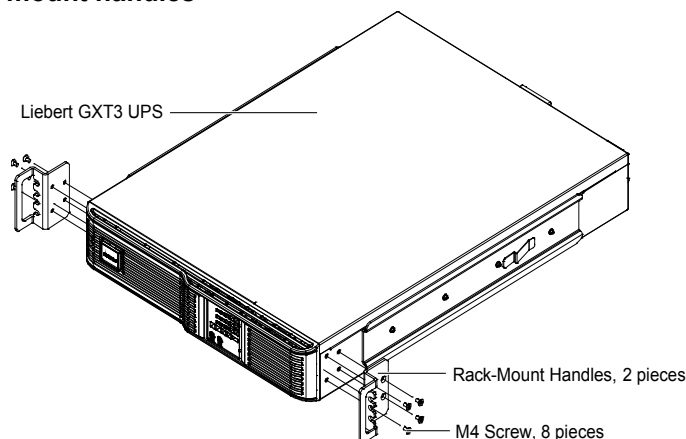
Figure 16 Installing rack-mount handles
