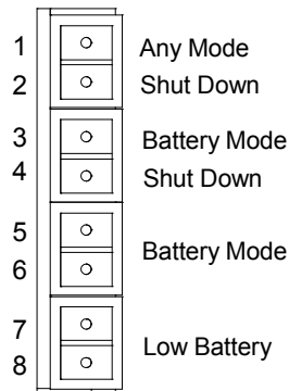
Figure 21 Terminal block communication pin layout
