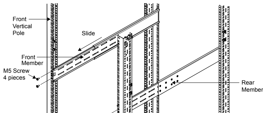
Figure 13 Installing front member of each slide rail assembly
