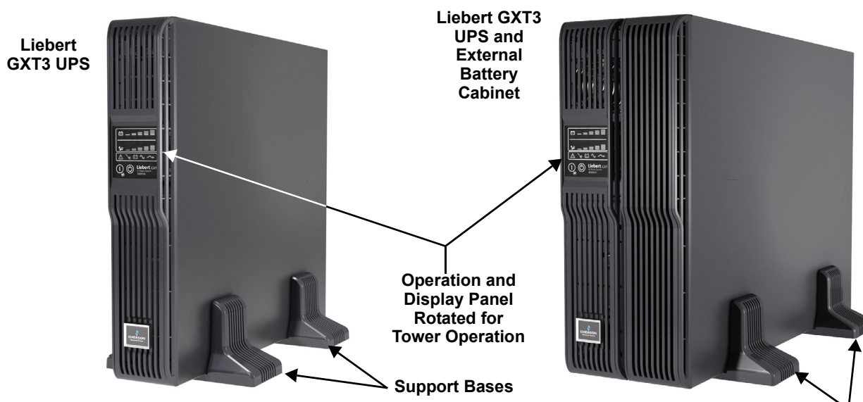
Figure 10 Tower installation
