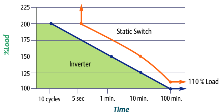
Overload capability of Liebert Npower UPS as a percent of nominal rating
