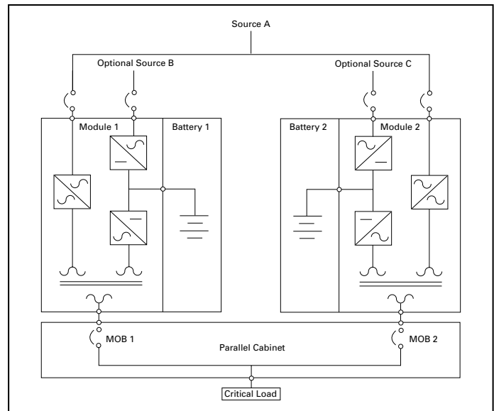
Typical 10 - 500 kVA Hot Sync Redundant Application
