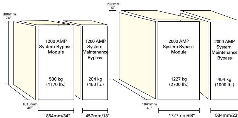
Powerware Hot Sync - Capacity
