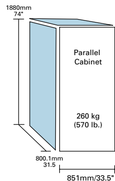
Powerware Hot Sync - Redundant
