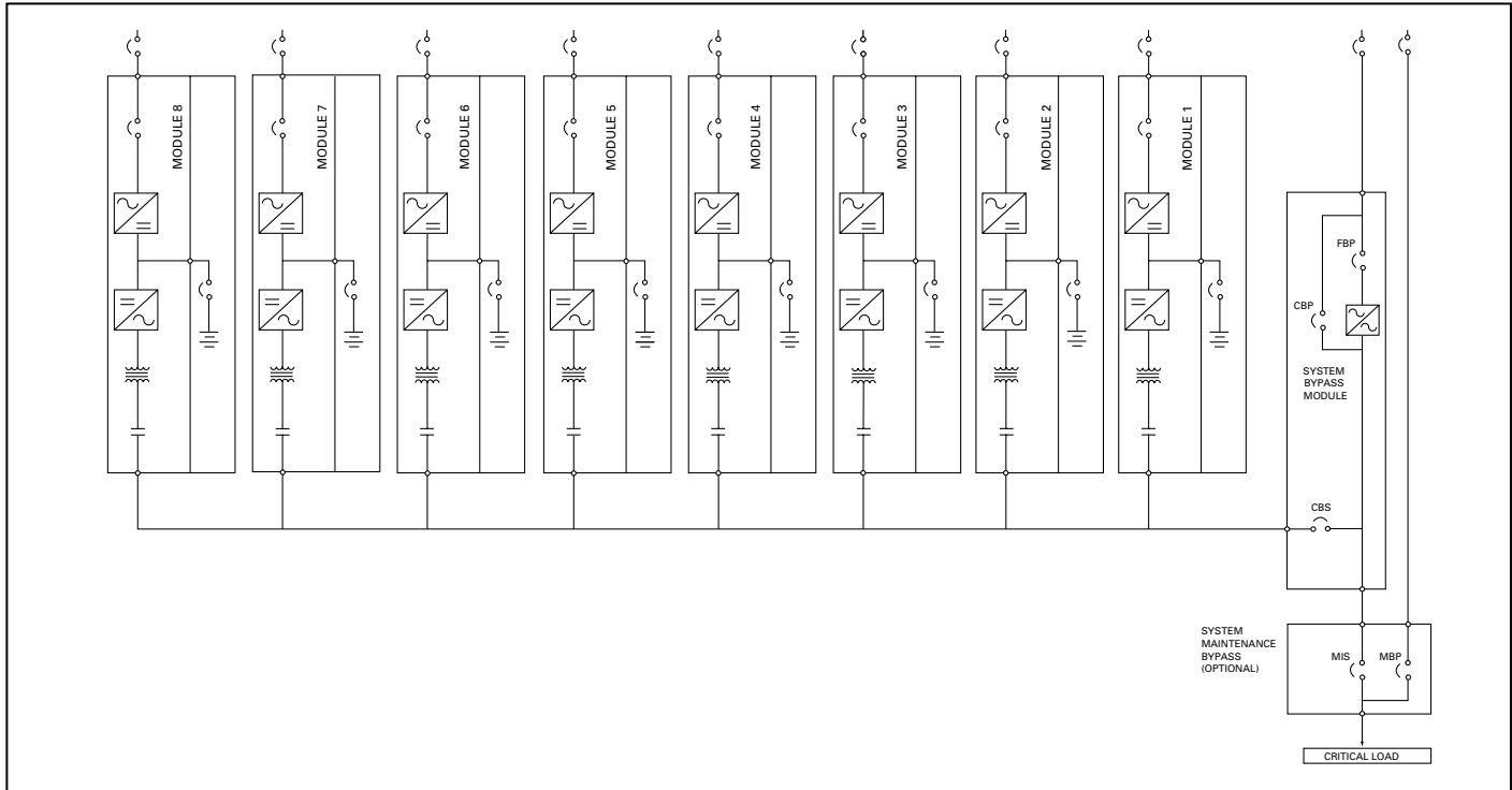
Typical Eaton 9315 200 - 750 kVA Hot Sync Capacity Application
