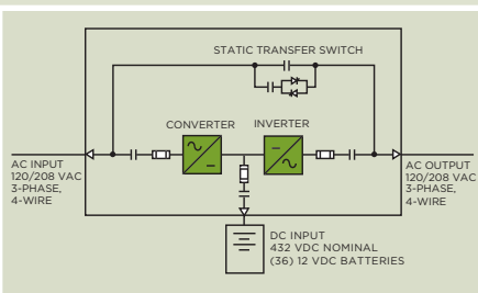
2033G ONE LINE DIAGRAM
