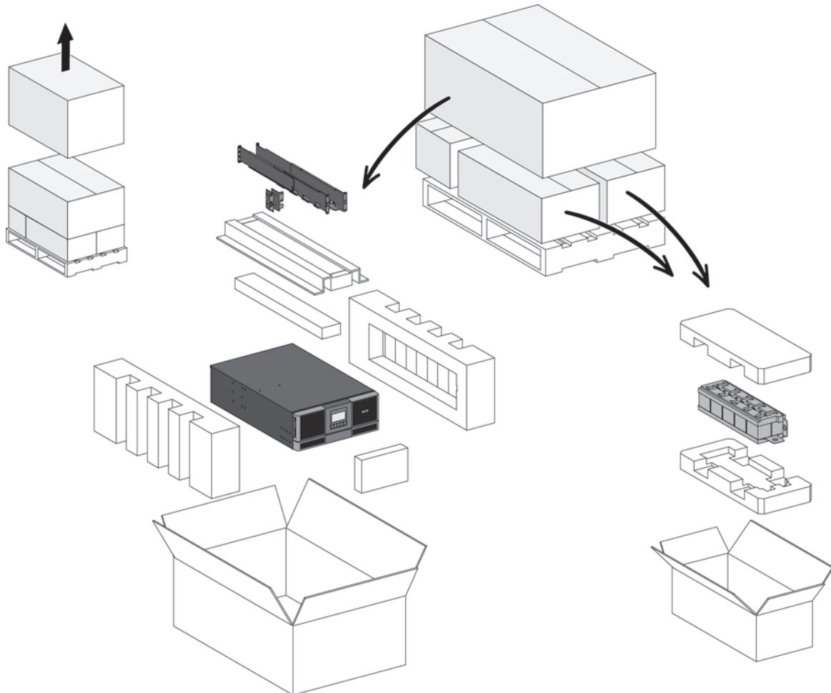
Unpacking UPS.
