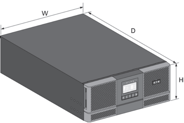
Rack installation
