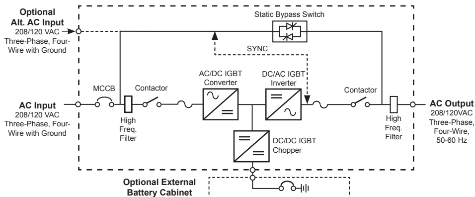
4300 Series UPS
