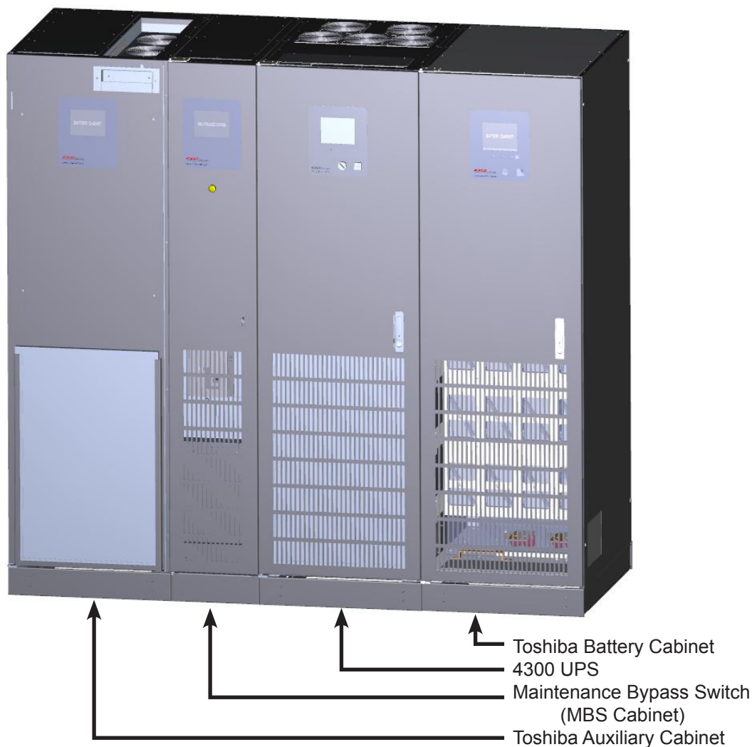
Figure 9-1 - 4300 Series System Assembly
