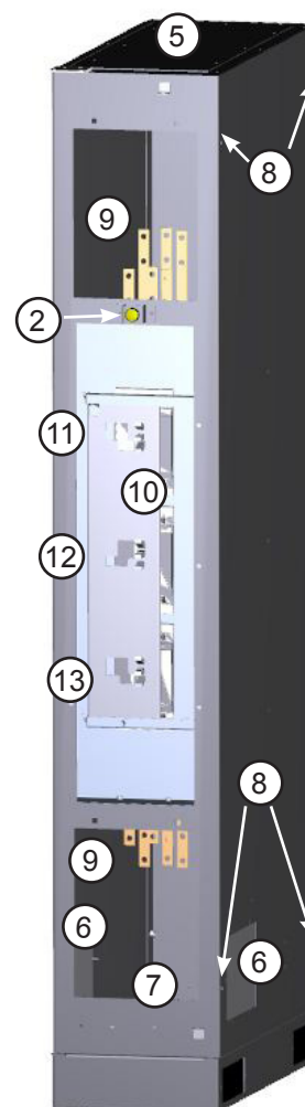
431M - Door Open (Dead Fronts Removed)
